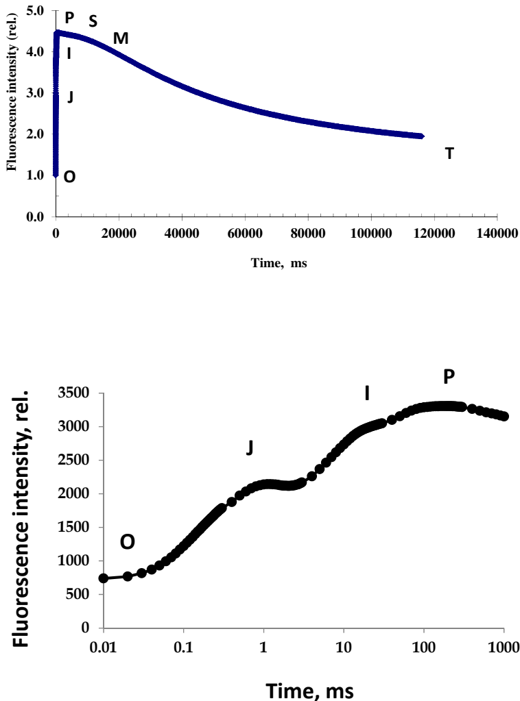
Fig. 6. Kautsky curve of a healthy green leaf and the expansion of the fast rise phase to the exponential 'OJIP' curve. The analysis of the OJIP curve gives rise to different parameters for the dark adapted state of the photosynthetic systems (details in text and also refer Strasser et al., 2004; Stirbet & Govindjee, 2011).
